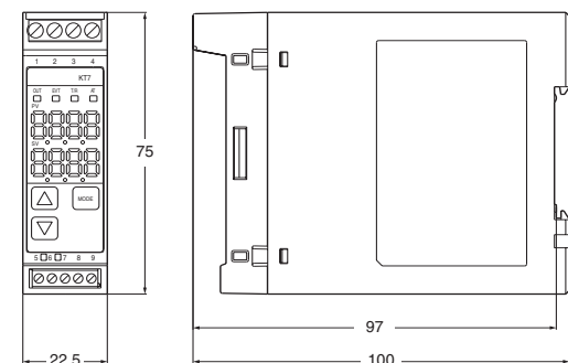
KT7 Series (unit: mm)
