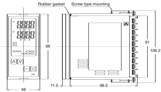
KT8 Series (unit: mm)
