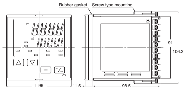
KT9 Series (unit: mm)
