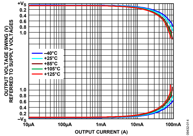
Figure 14. Output Voltage Swing vs. Output Current vs. Temperature, V_S = \pm 5\text{ V} and +5\text{ V}
