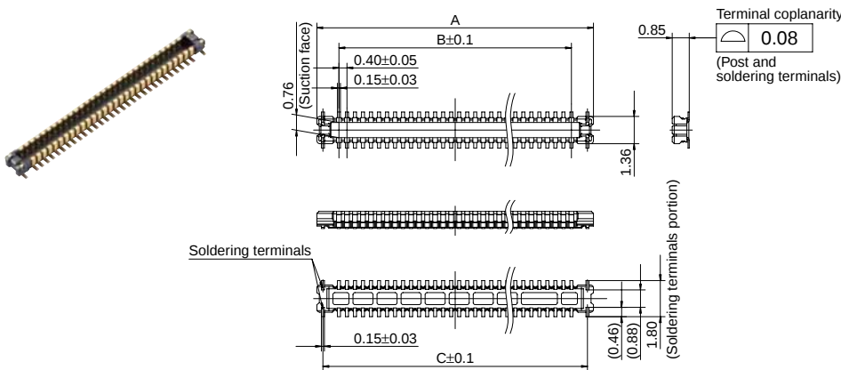
Dimension table (mm)
