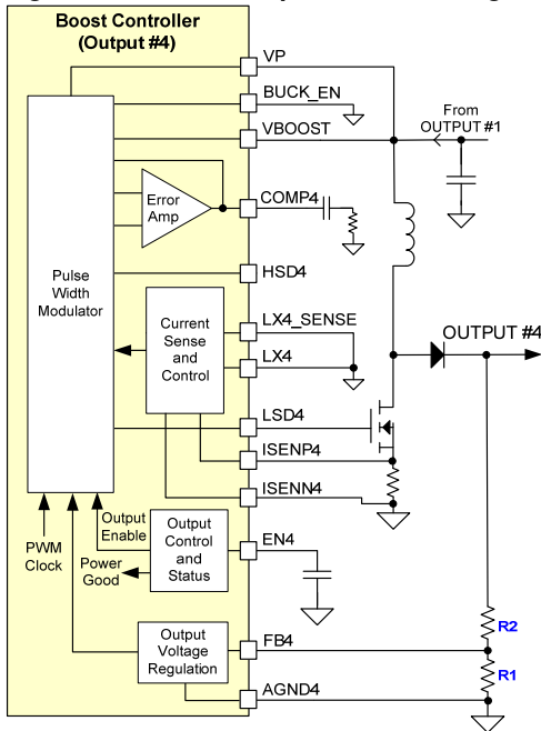
Figure 14 - Power Output #4 Block Diagram - BOOST
