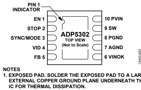
Figure 3. Pin Configuration
