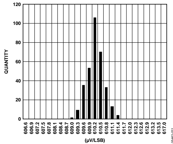
Figure 21. DAC Gain Distribution at 25°C/3.3 V
