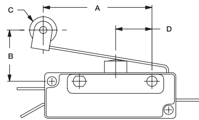
FIG. 8 Leaf Roller
