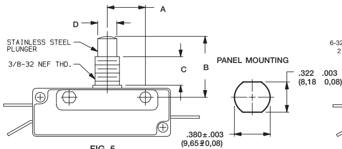
FIG. 5 High Overtravel Plunger
