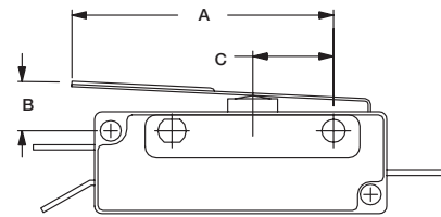
FIG. 2 Leaf
