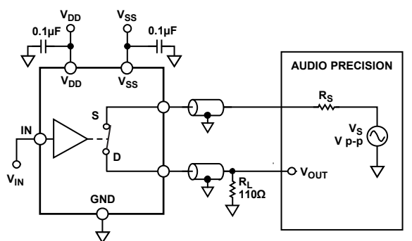
Figure 36. THD + Noise
