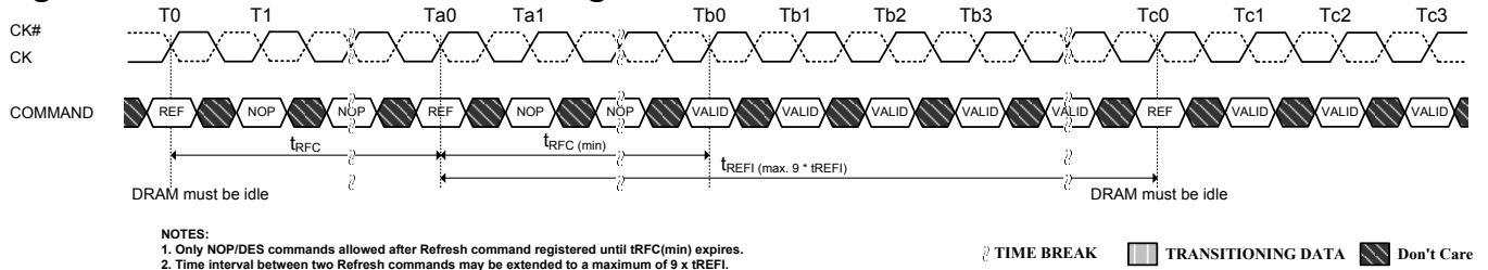
Figure 53. Refresh Command Timing
