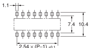
Mounting pads (top view)
