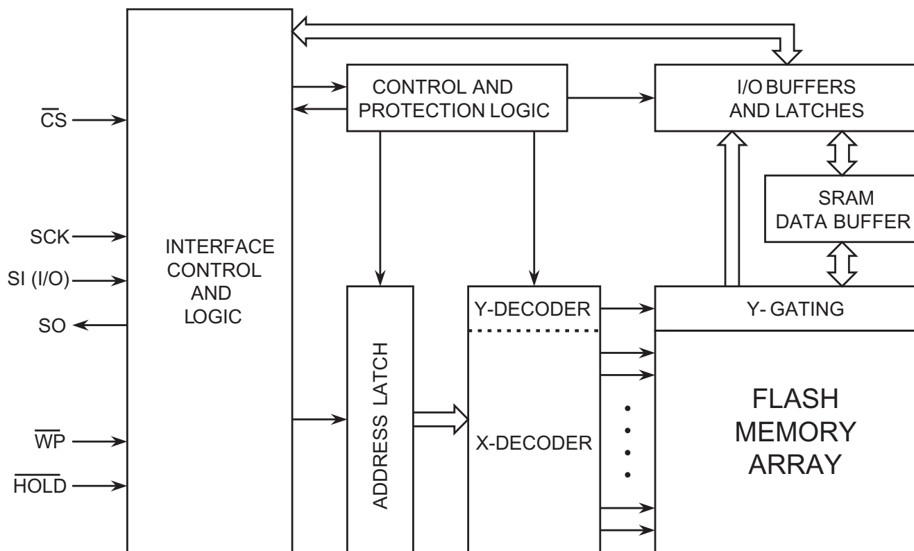
Figure 3-1. Block Diagram
