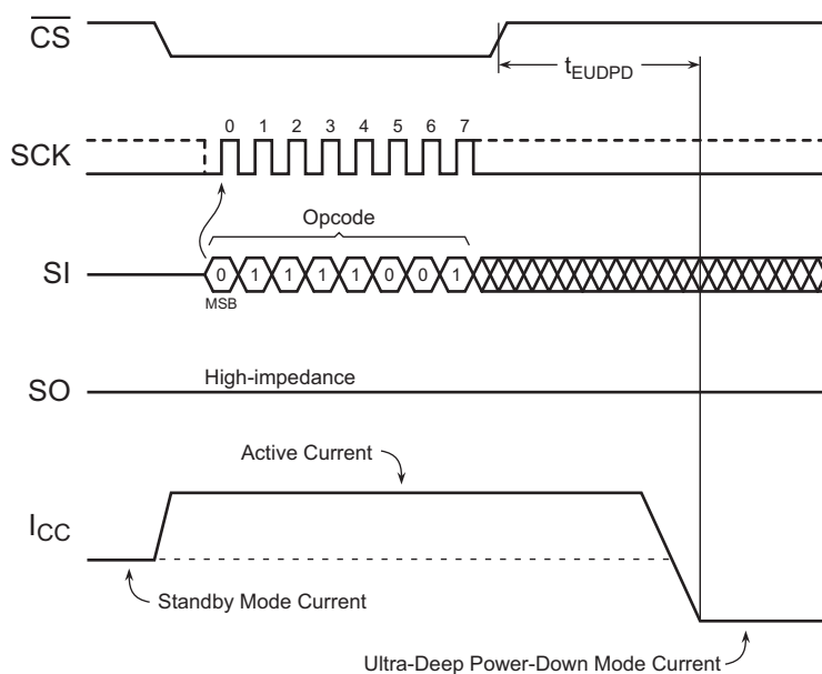
Figure 12-5. Ultra-Deep Power-Down
