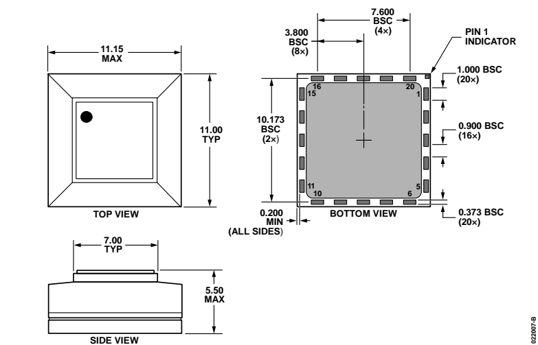
Figure 24. 20-Terminal Stacked Land Grid Array [LGA] (CC-20-1) Dimensions shown in millimeters
