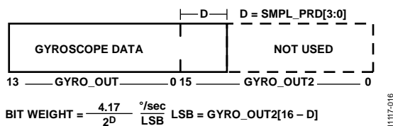
Figure 15. Gyroscope Output Format
