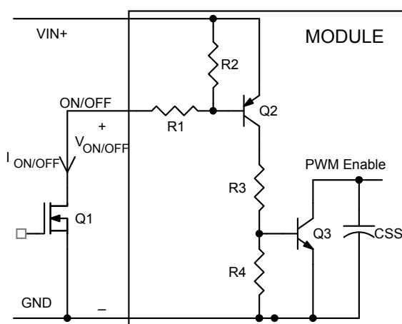
Figure 28. Circuit configuration for using positive logic On/Off.
