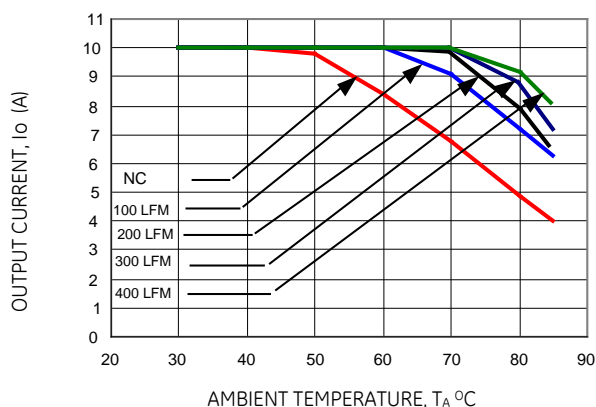
Figure 19. Derating Output Current versus Local Ambient Temperature and Airflow ( V_{in} = 12.0 , V_o=0.75 Vdc).
