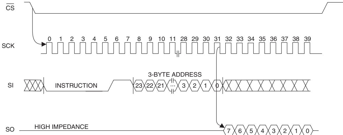
Figure 8. READ Timing
