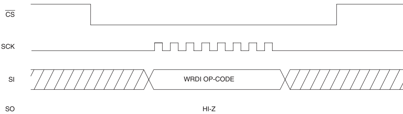
Figure 5. WRDI Timing
