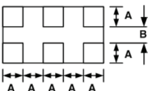
Chip Antenna Soldering Pad Dimension
