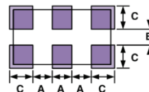
PCB Soldering Land Dimension
