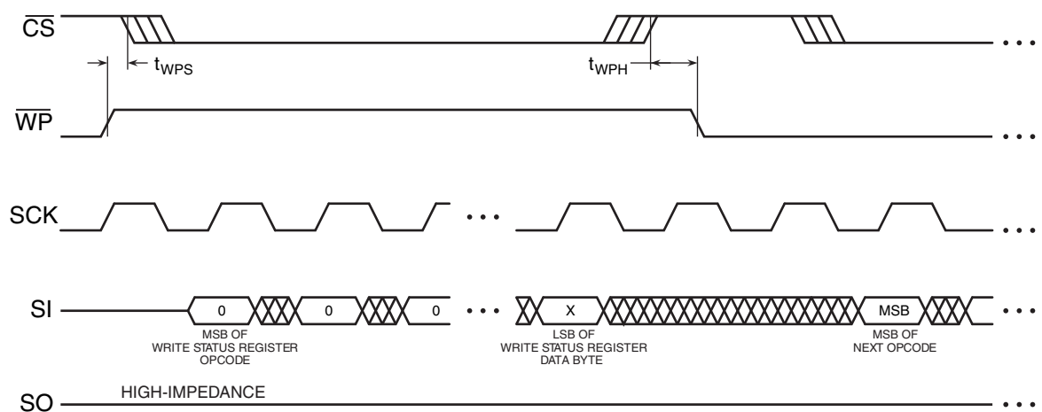
Figure 15-3. \overline{WP} Timing for Write Status Register Command When BPL = 1
