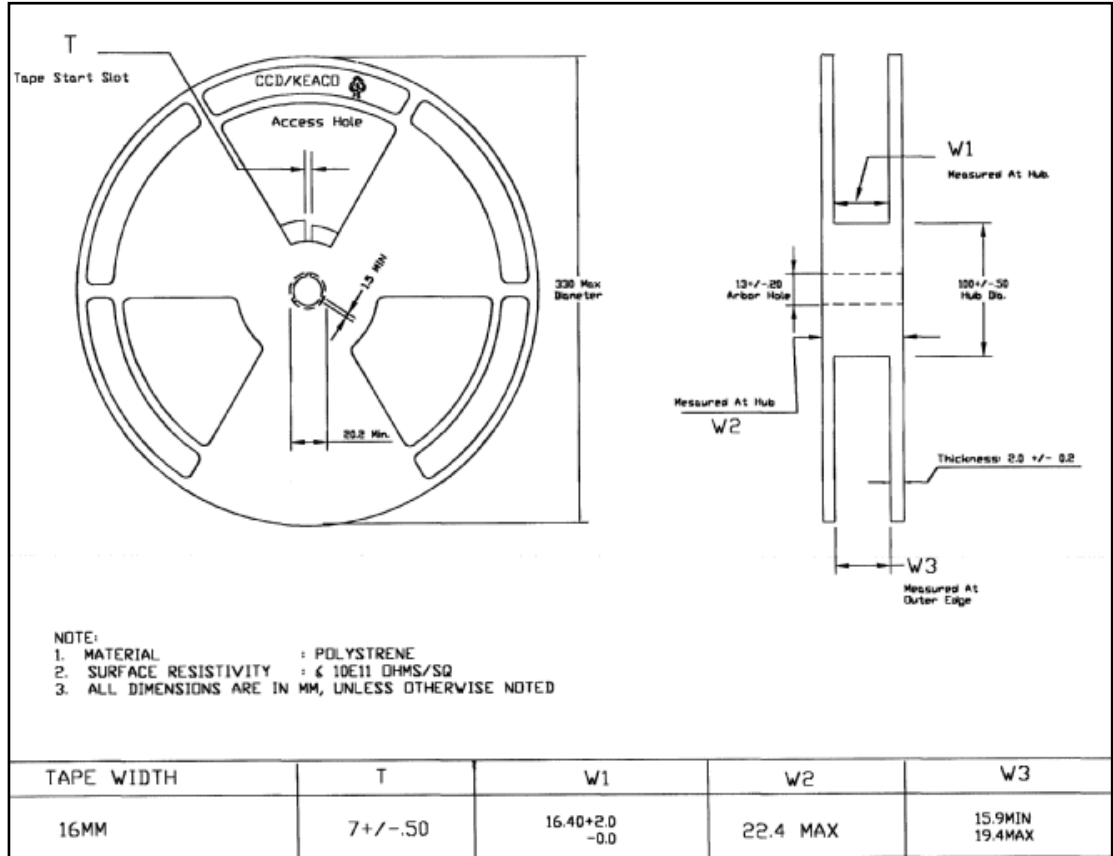
Figure 38. Reel Information.
