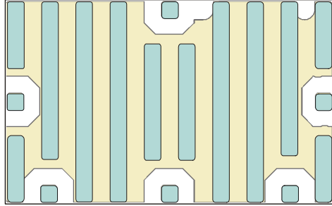
Figure 33. Solder Stencil Overlaid on ACFM-7101 Bottom Metal Pattern.
