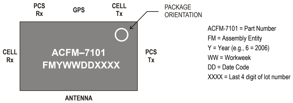
Figure 32. Package Marking.
