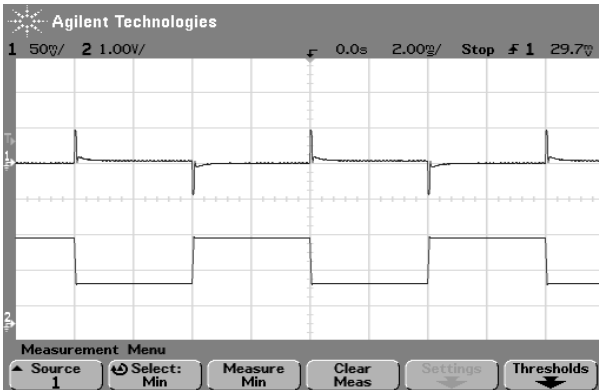
Fig.35 Typical transient response to step decrease in load from 50% to 25%, room temperature, 48Vdc input ( \Delta I_o/\Delta t = 0.1A/1\mu s ) of AGQ100-48S1V8
