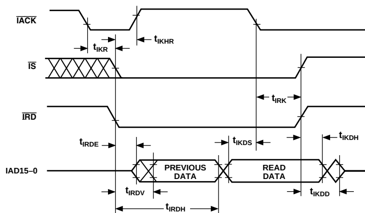
Figure 28. IDMA Read, Long Read Cycle
