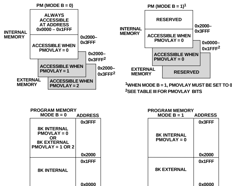
Figure 4. Program Memory
