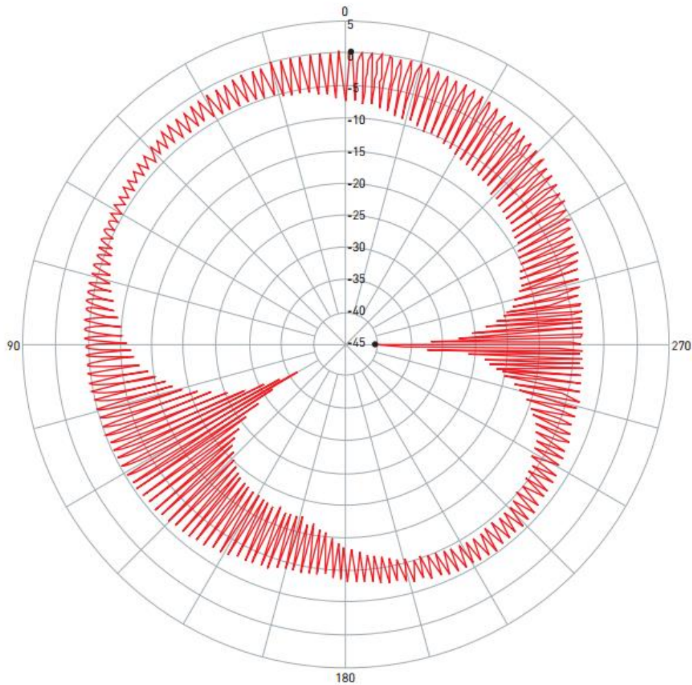
1575.42MHz Axial Ratio
