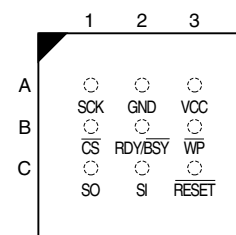
Figure 2-4. CBGA Top View through Package
