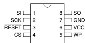
Figure 2-2. 8-SOIC
