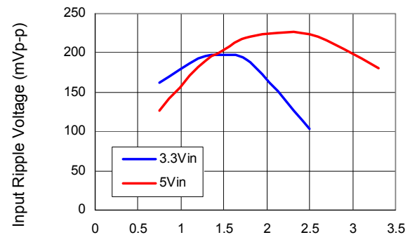
Figure 27. Input ripple voltage for various output with 2x150 µF polymer and 2x47 µF ceramic capacitors at the input (full load).
