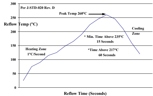
Figure 37. Recommended linear reflow profile using Sn/Ag/Cu solder.
