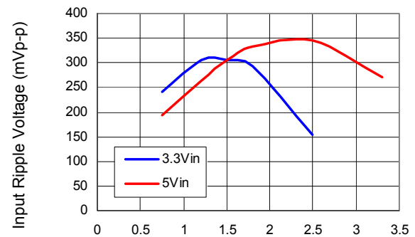
Figure 26. Input ripple voltage for various output with 1x150 µF polymer and 1x47 µF ceramic capacitors at the input (full load).
