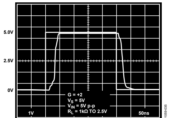
Figure 37. Overdrive Recovery
