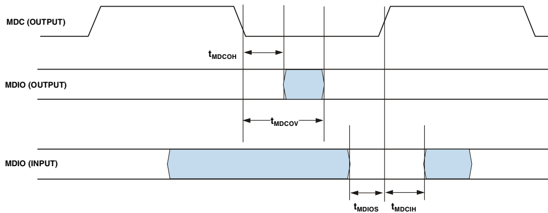
Figure 41. 10/100 Ethernet MAC Controller Timing: MII Station Management
