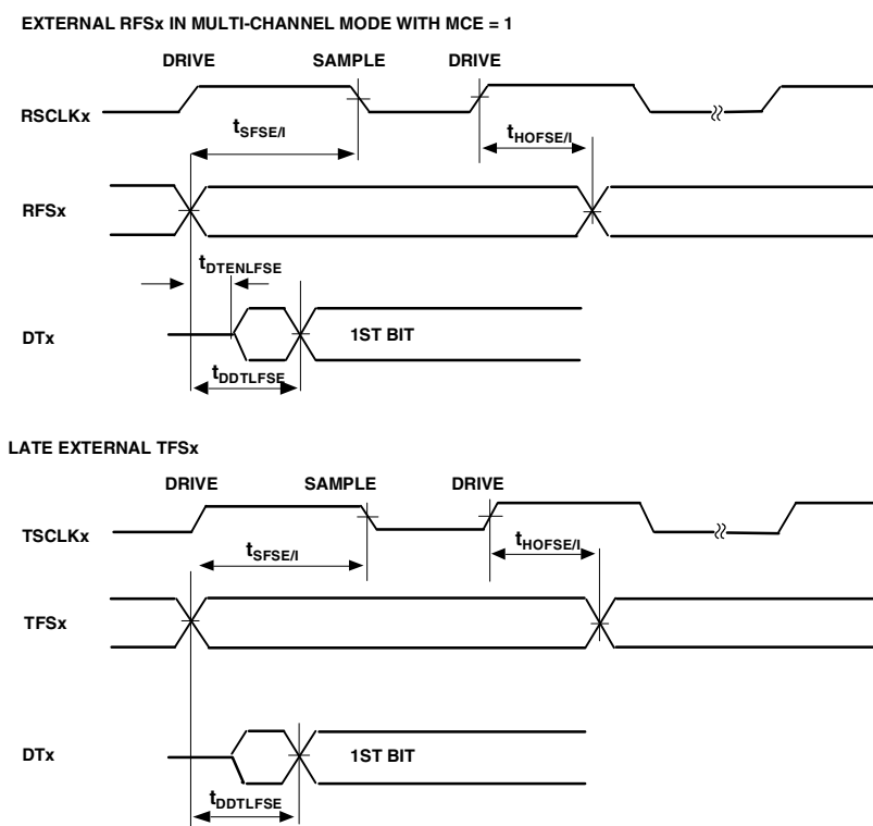
Figure 26. Serial Ports — External Late Frame Sync
