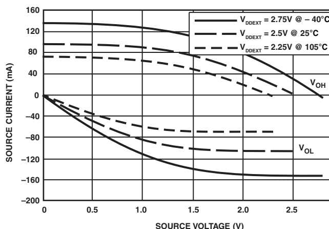
Figure 47. Driver Type B Current ( 2.5V_{DDEXT}/V_{DDMEH} )
