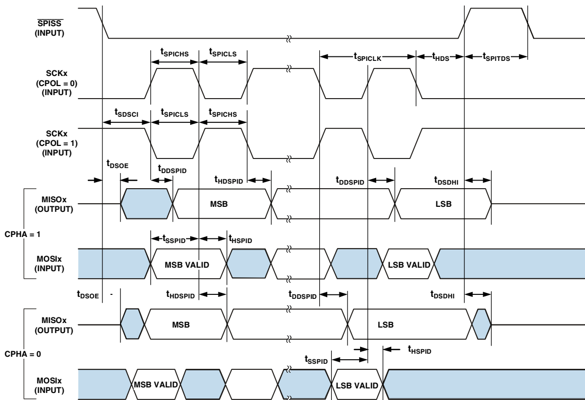
Figure 28. Serial Peripheral Interface (SPI) Port—Slave Timing
