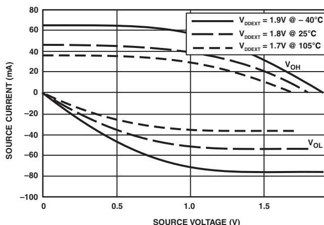
Figure 48. Driver Type B Current ( 1.8V_{DDEXT}/V_{DDMEH} )
