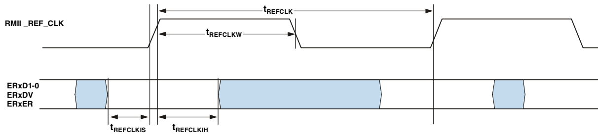
Figure 38. 10/100 Ethernet MAC Controller Timing: RII Receive Signal
