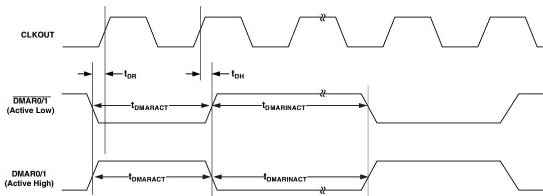
Figure 19. External DMA Request Timing
