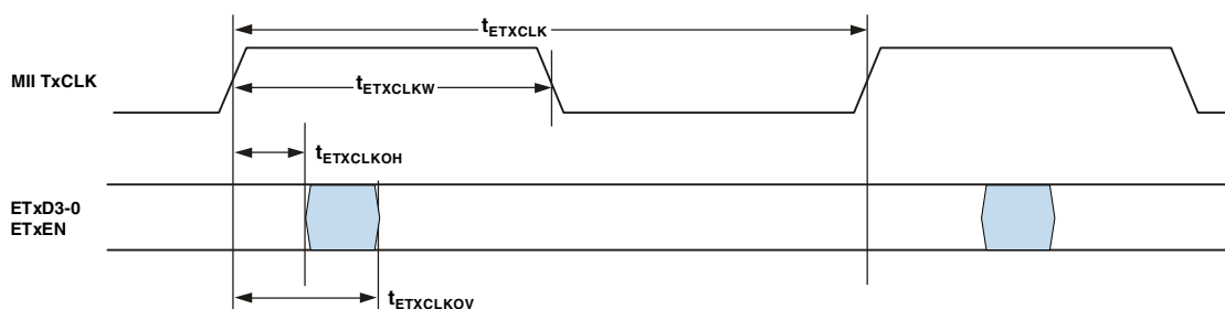
Figure 37. 10/100 Ethernet MAC Controller Timing: MII Transmit Signal
