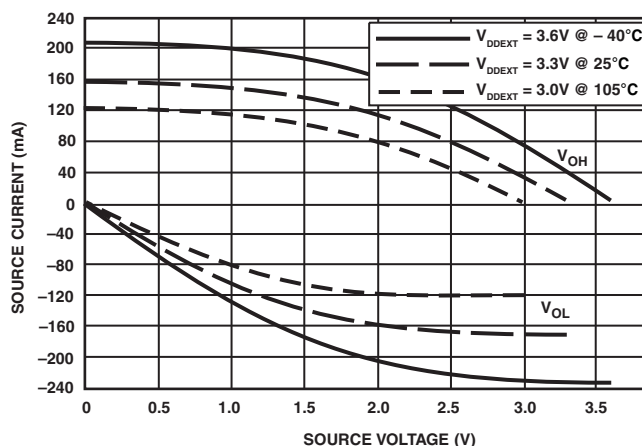
Figure 46. Driver Type B Current ( 3.3V_{DDEXT}/V_{DDMEH} )
