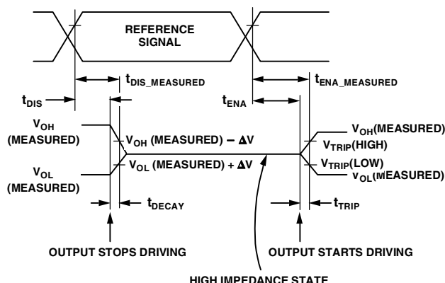
Figure 59. Output Enable/Disable
